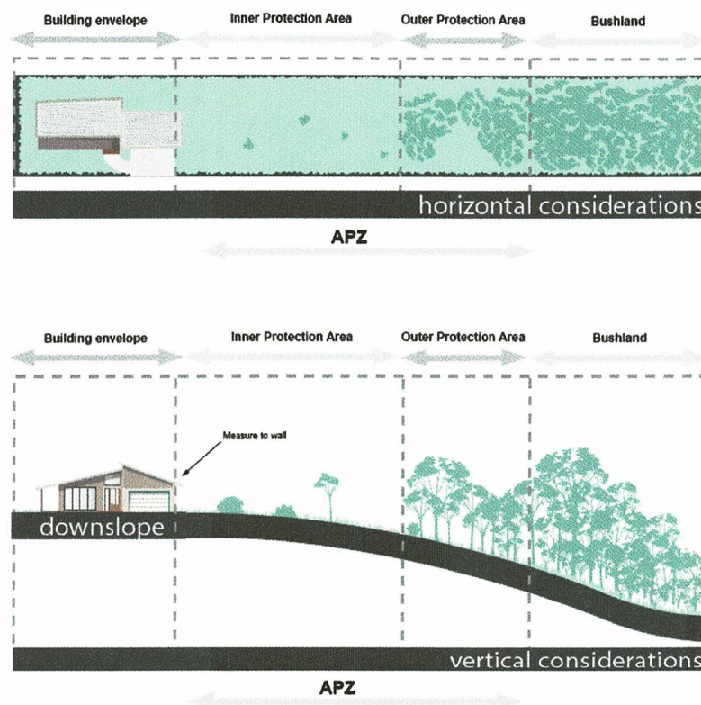
Typical Inner and Outer Protection Areas.
