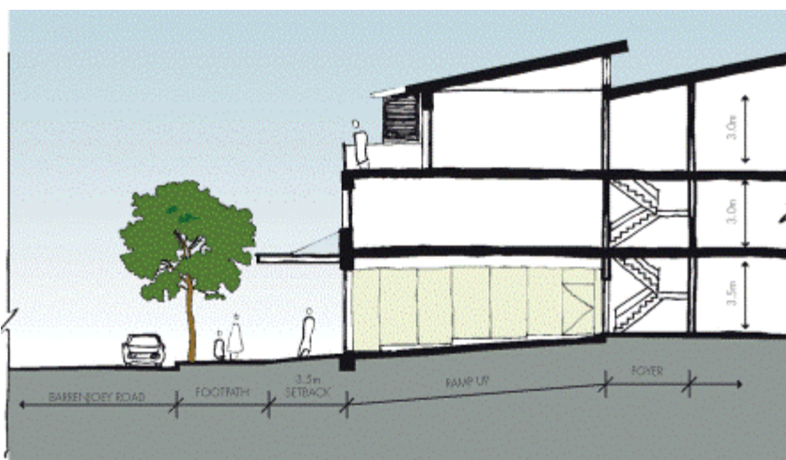
Figure 2. Design solutions for flooding in Newport Commercial Centre
