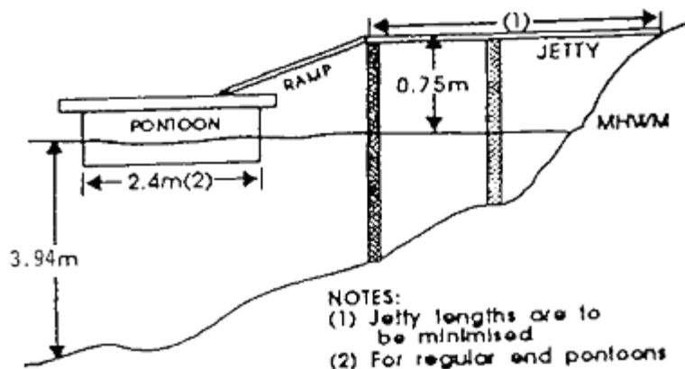
Diagram 2: Maximum Dimensions for Berthing Areas -Perpendicular to Shore (As per Department of Infrastructure Planning and Natural Resources requirements)
