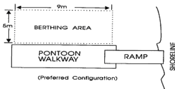
Diagram 3B: Maximum Dimensions for Berthing Areas - Parallel to Shore
