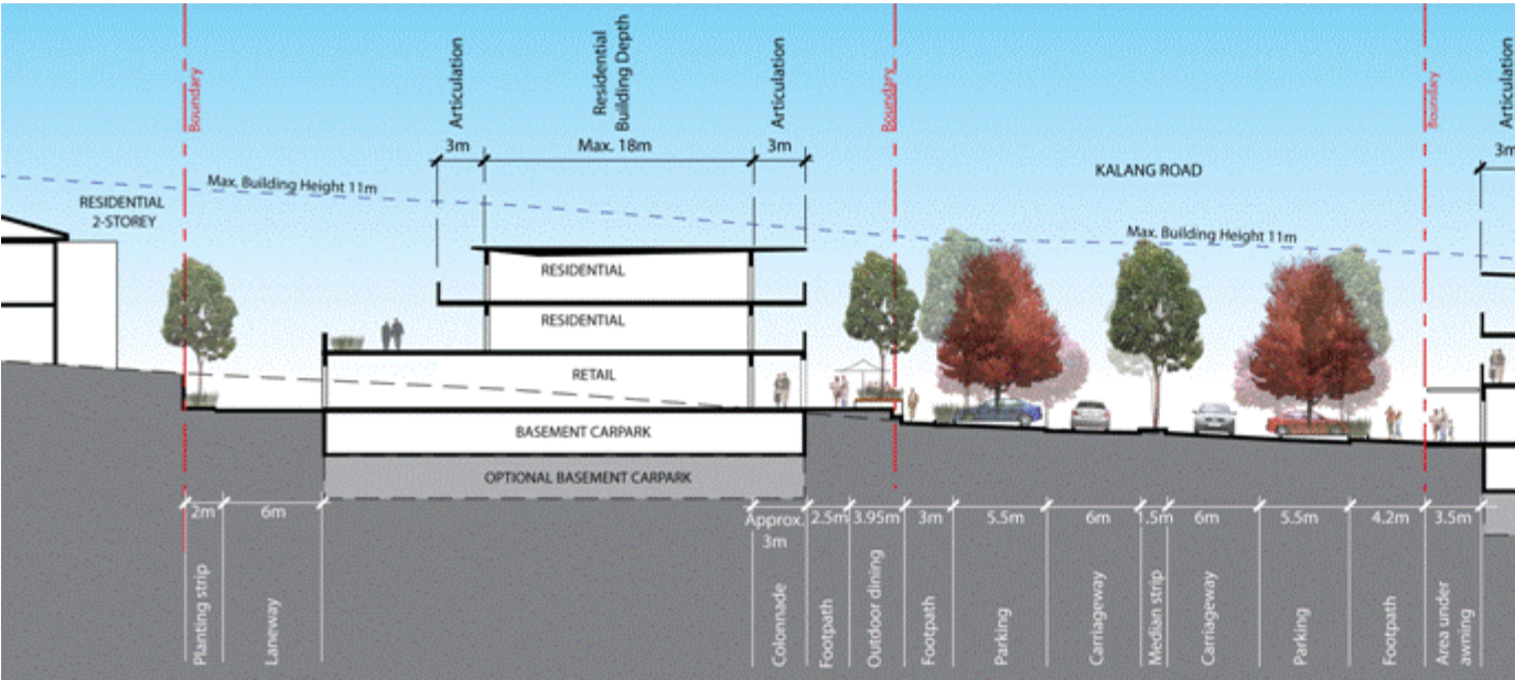
Section B:B through Elanora Heights Village Centre - South (south of St Andrews Gate)
