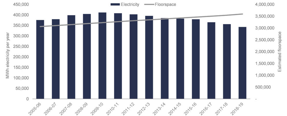
Figure 10: Total electricity consumption for Pyrmont and Ultimo compared to floorspace growth (Source: Ausgrid and City of Sydney FES)
