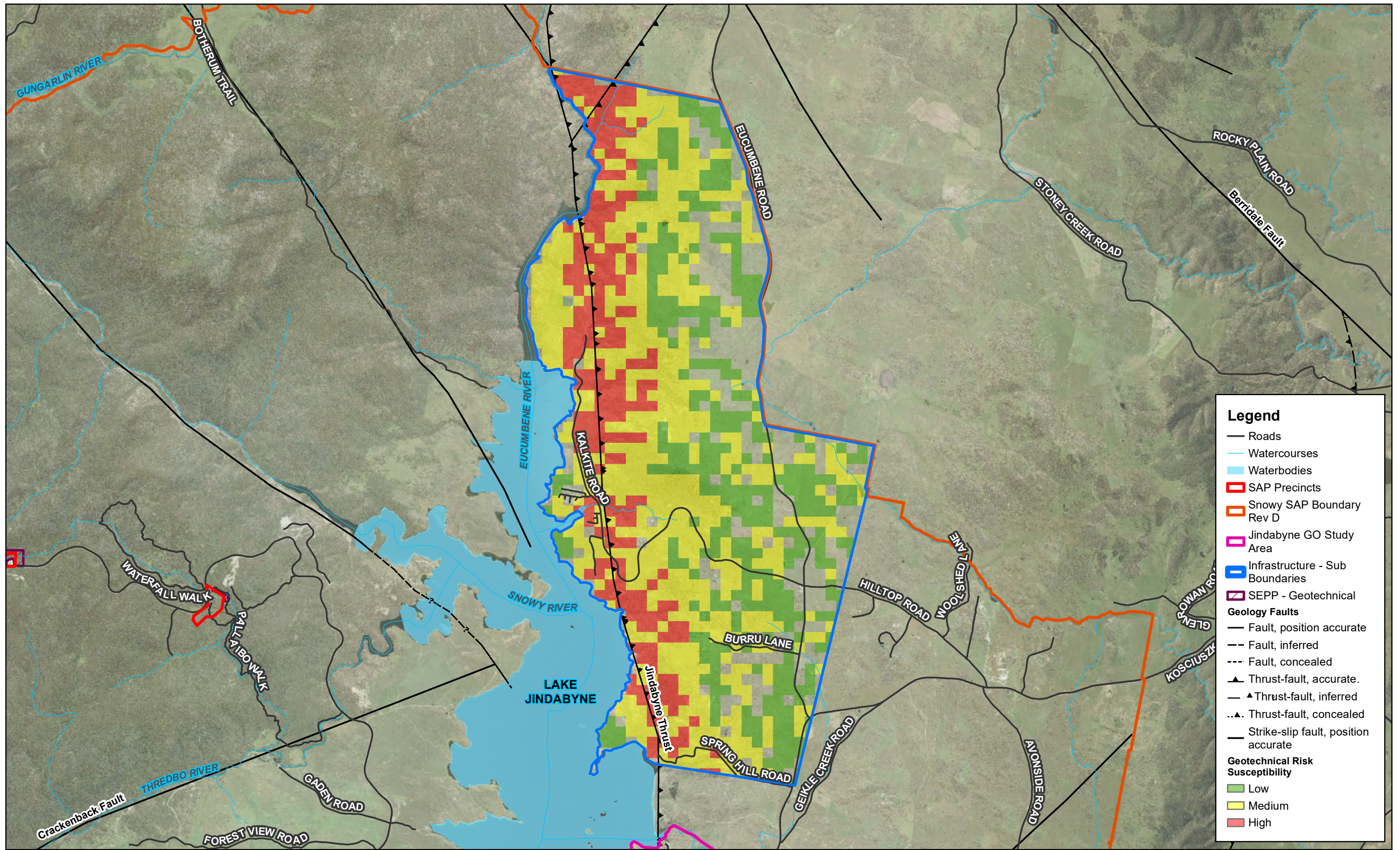
Snowy SAP Figure 1 Geotechnical Risk Susceptibility - Eastern Lake Jindabyne Area
