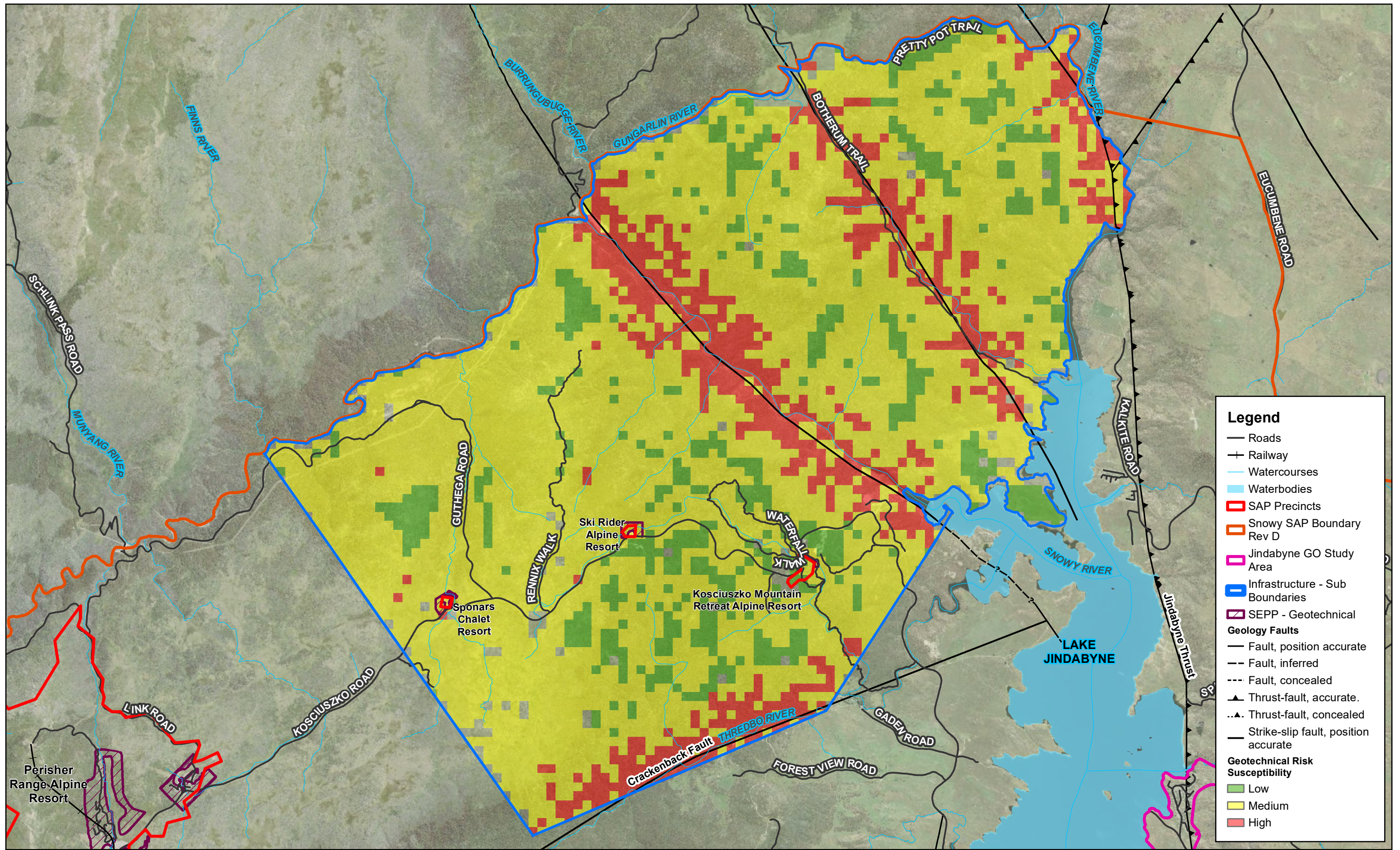
Snowy SAP Figure 1 Geotechnical Risk Susceptibility - Kosciuszko Road Area
