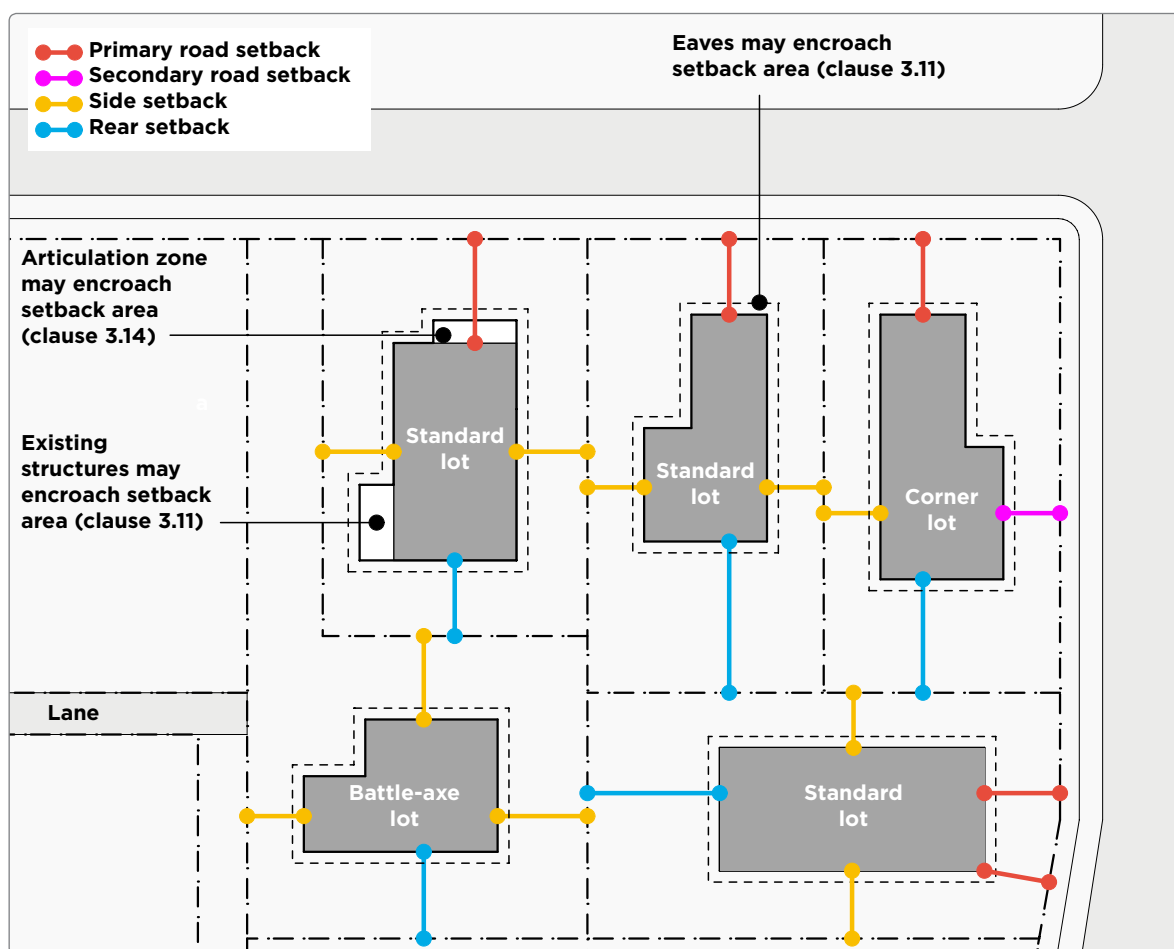
SETBACK TYPES
