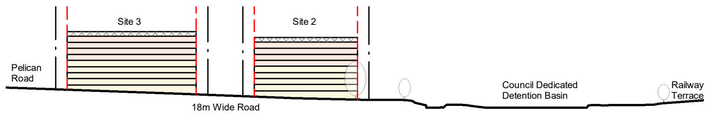
Building Envelope Section A2
