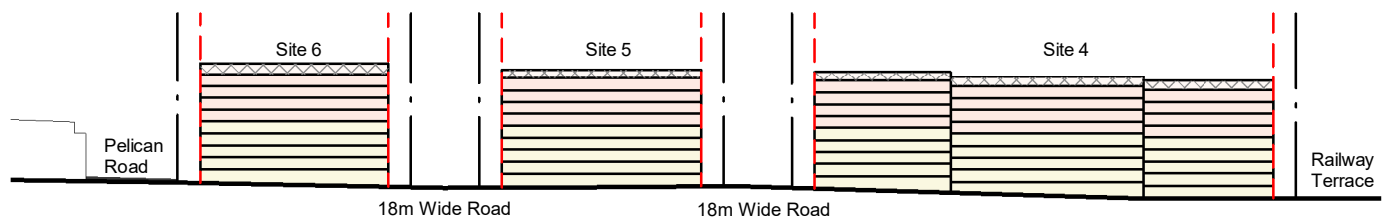
Building Envelope Section A3
