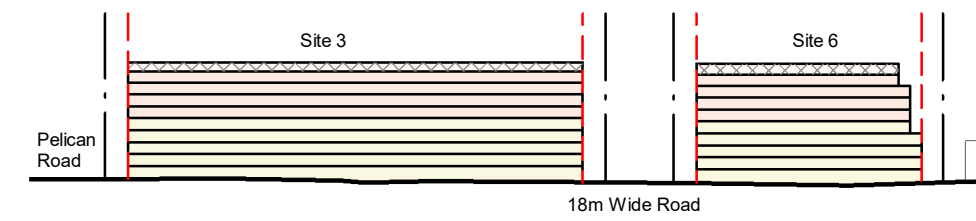
Building Envelope Section B3
