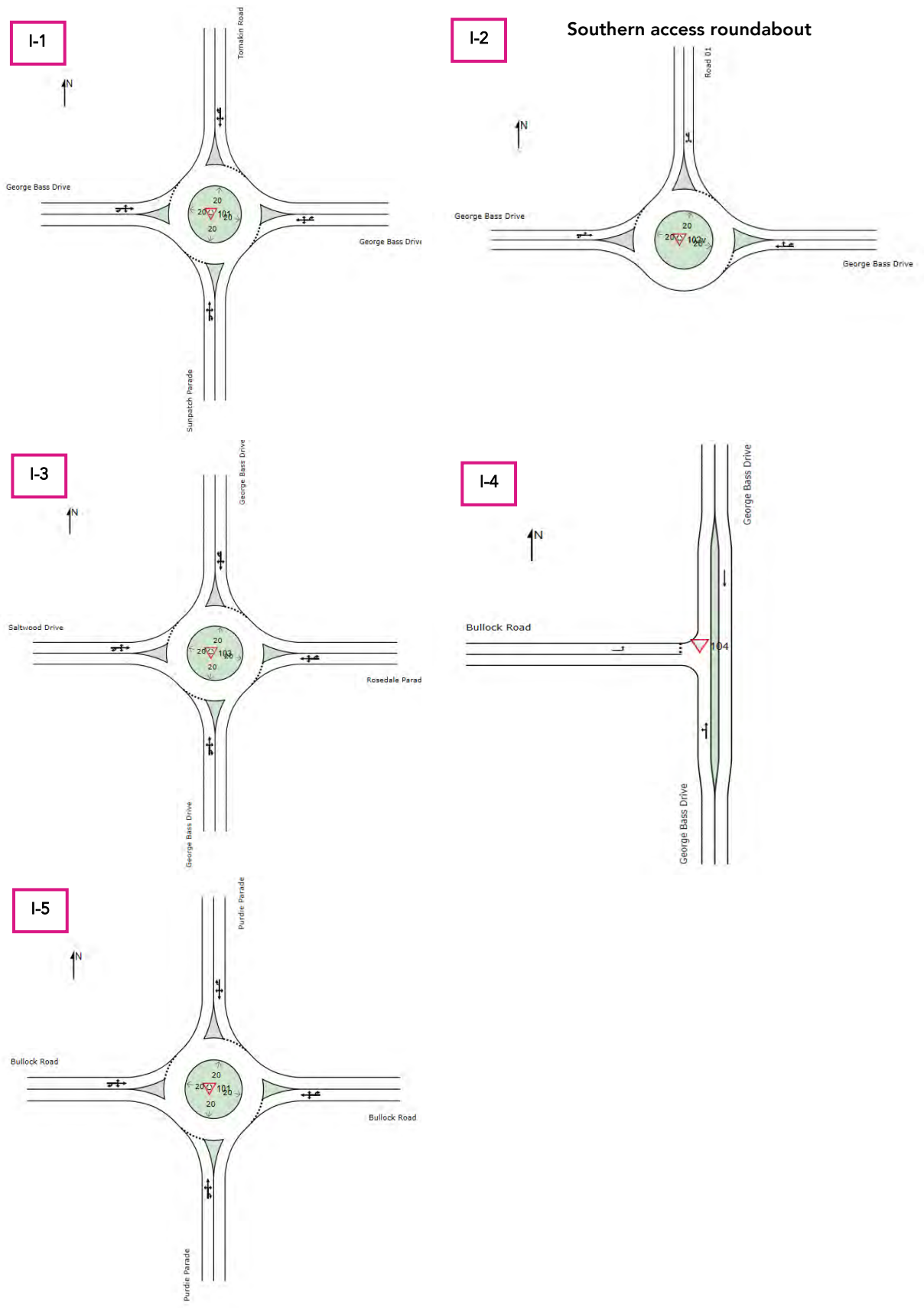
Figure 18 – Base SIDRA model
