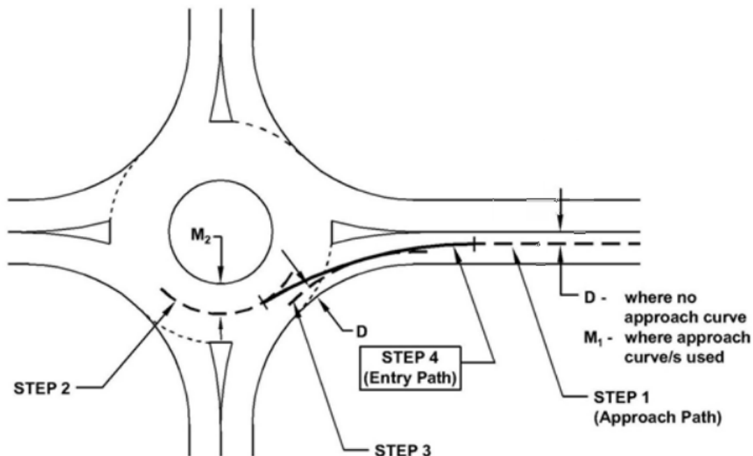
Figure 22 – Steps to construct the entry path (Source : Austroads Guide to Road Design Part 4B)
