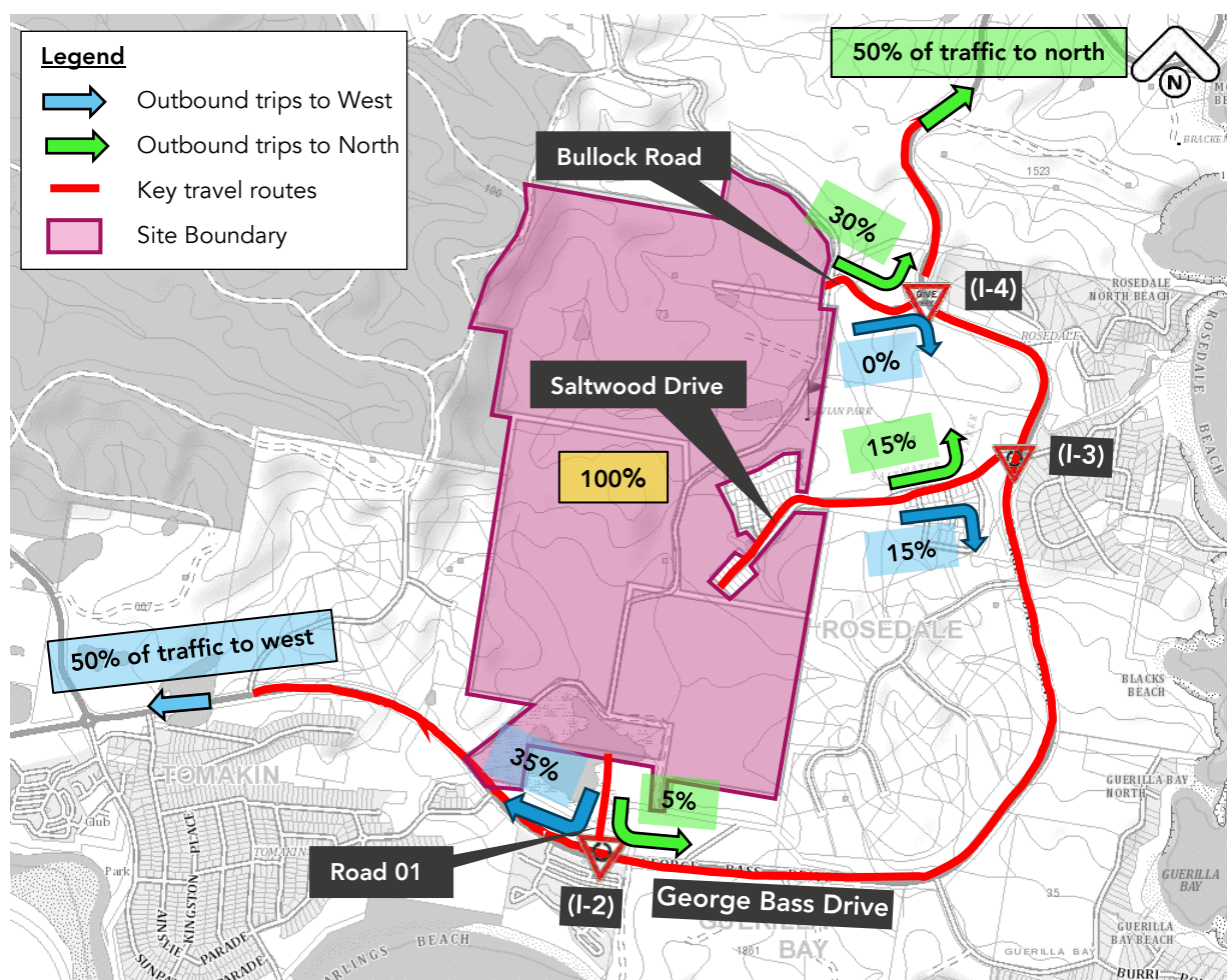
Figure 17 – Proposed outbound trip distribution
