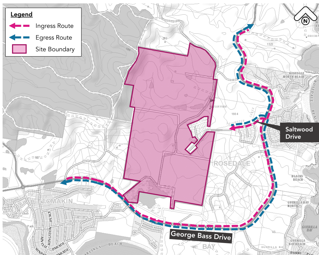
Figure 24 – Construction Vehicle Routes
