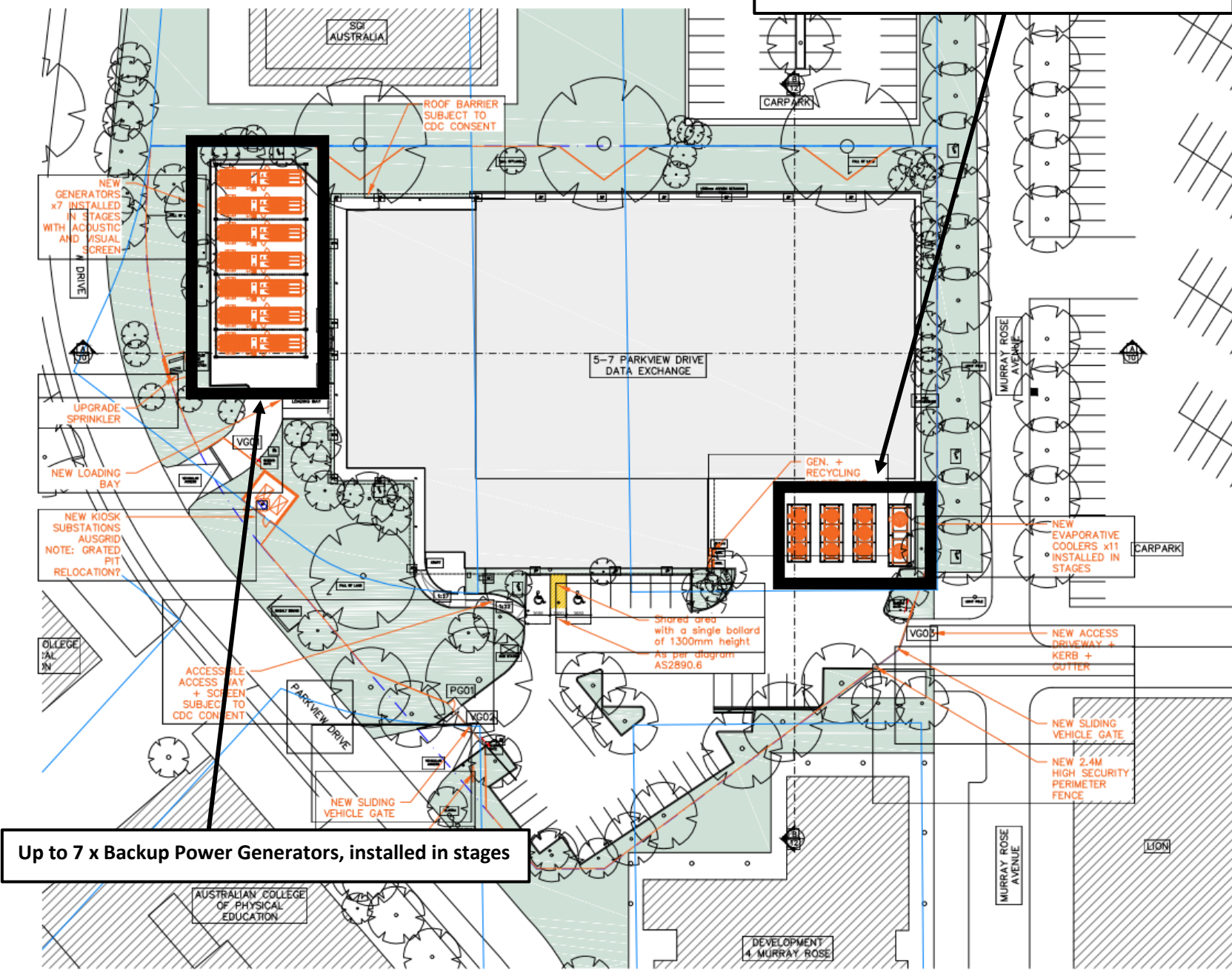
Figure 2-2: Site Layout Plan
