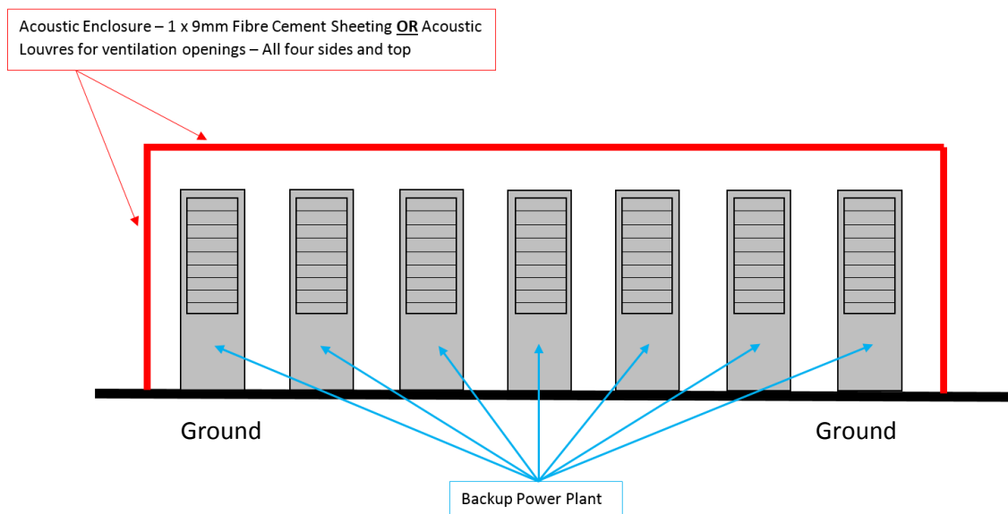
Figure 4-1: Section View of the Indicative Backup Power Plant Enclosure
