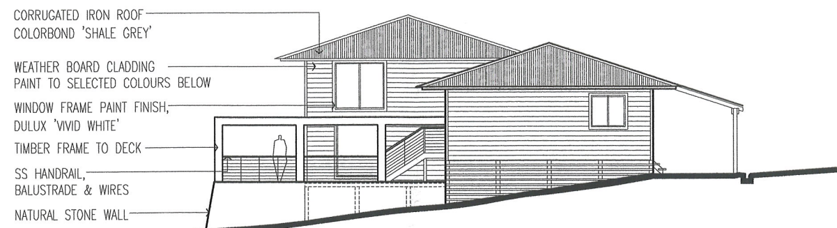
1 TYPE 1 EAST ELEVATION DA-05 TYPE 2 SIMILAR
