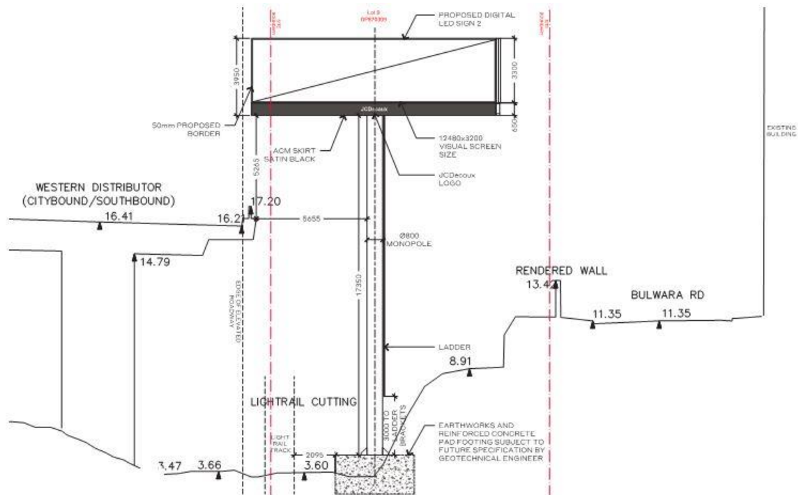
Figure 6.4 – Elevation sign 2
