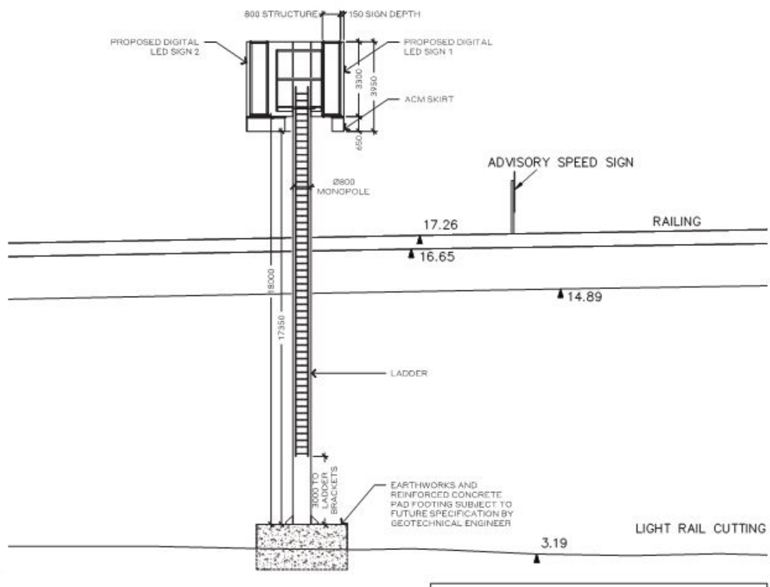
Figure 6.5 – Side elevation
