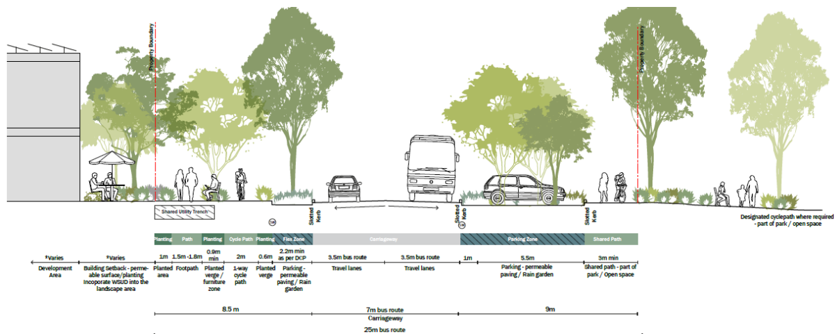
Figure 7-8 Typical <25m local street cross section (at a park edge)
