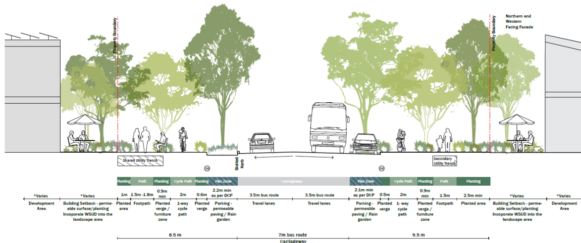
Figure 7-7 Typical 25m local collector corridor cross section
