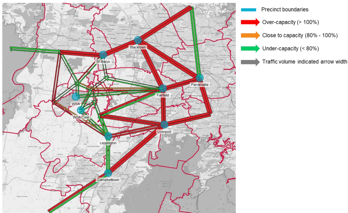
Figure 8-21 Wider 2056 road network capacity assessment
