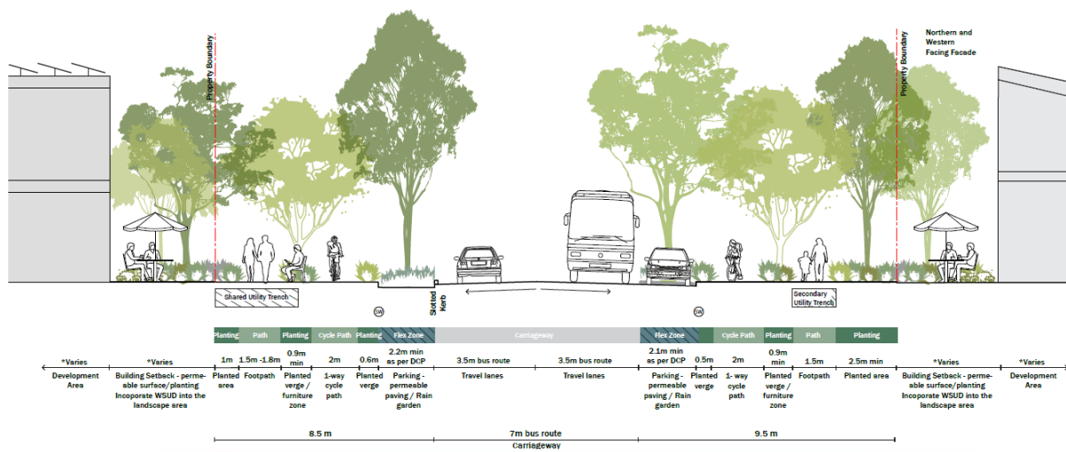
Figure 7-9 Typical <25m industrial street cross section
