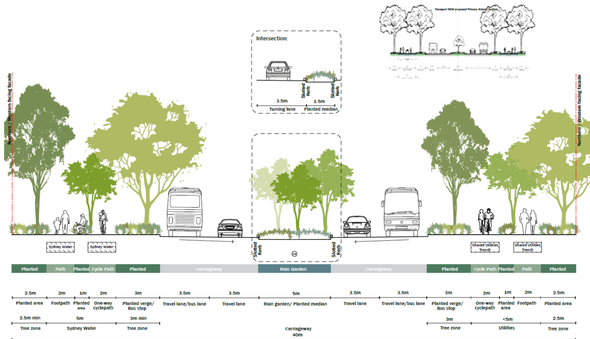
Figure 7-5 Typical 40m corridor cross section
