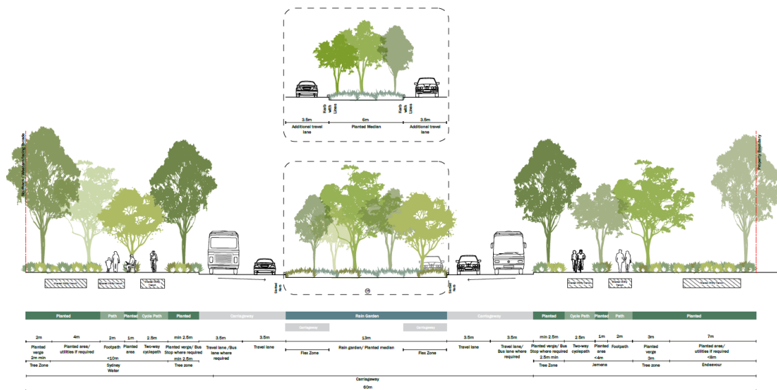
Figure 7-4 Typical 60m corridor cross section
