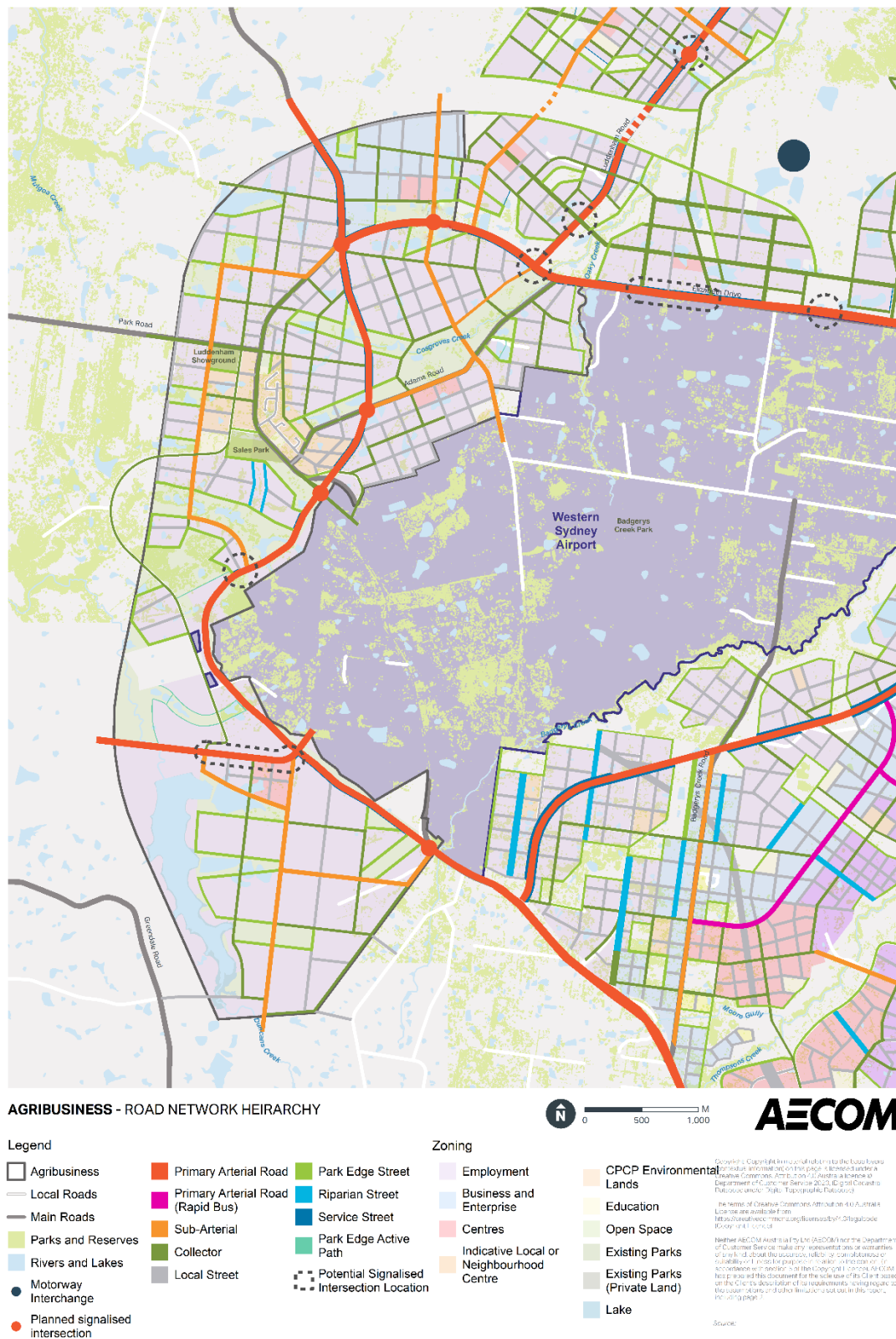
Figure 7-28 Agribusiness proposed road network
