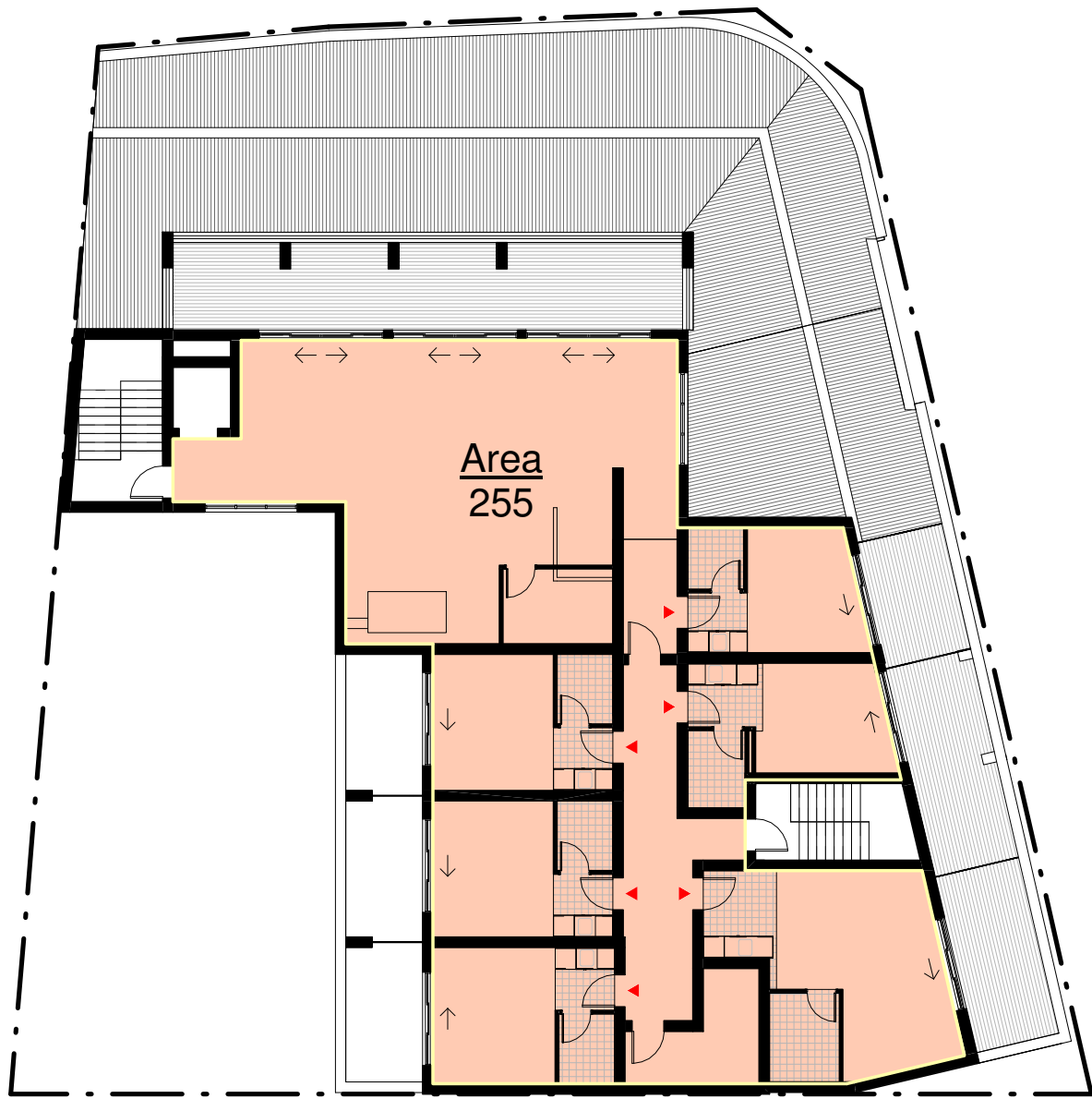
5 | Level 4 1:200
