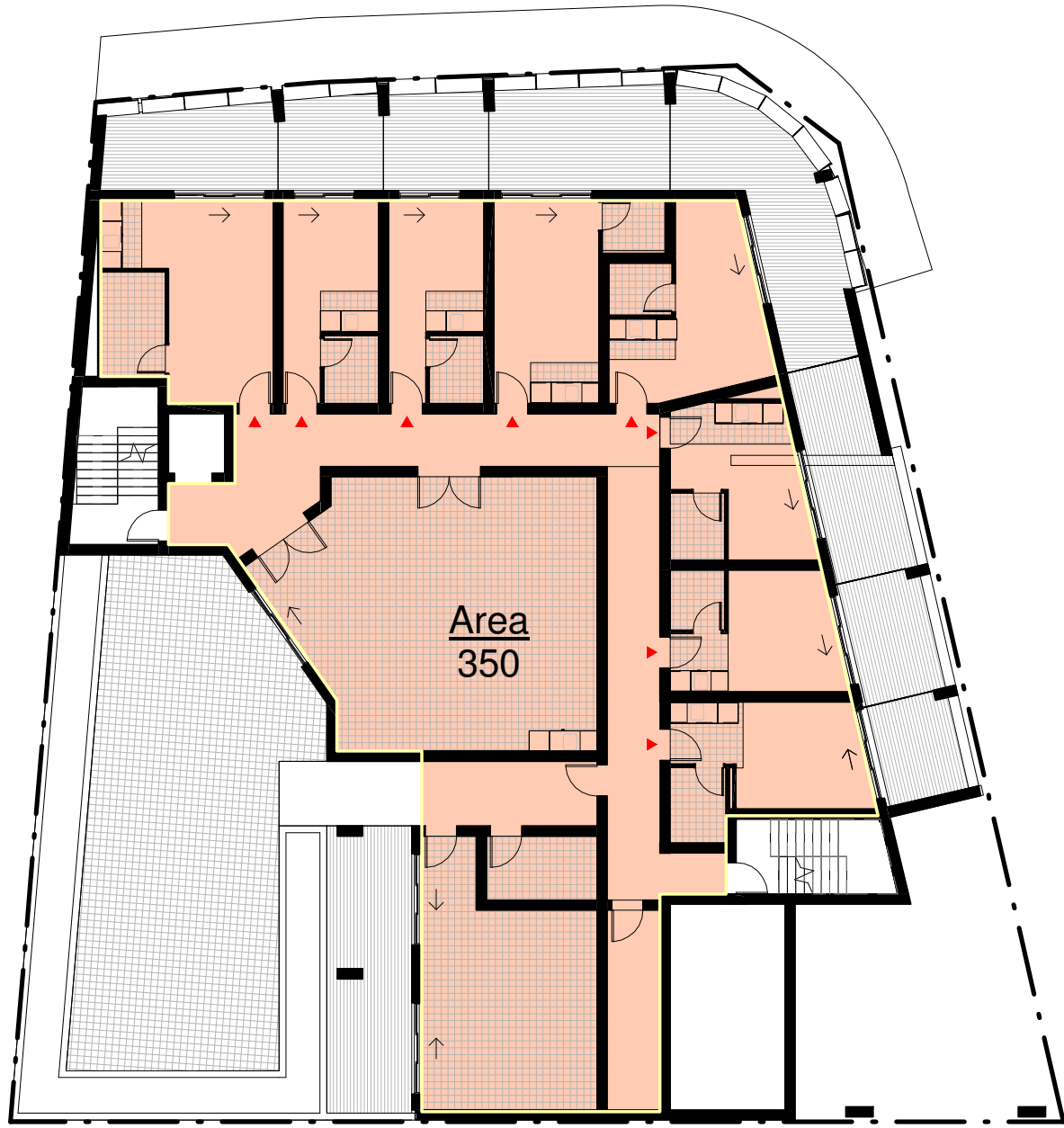
2 | Level 1 1:200
