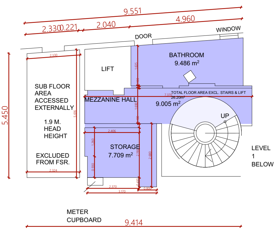
MEZZANINE
